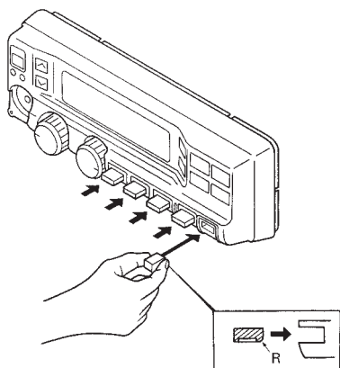
Fig. 1-4 Keytop insertion
