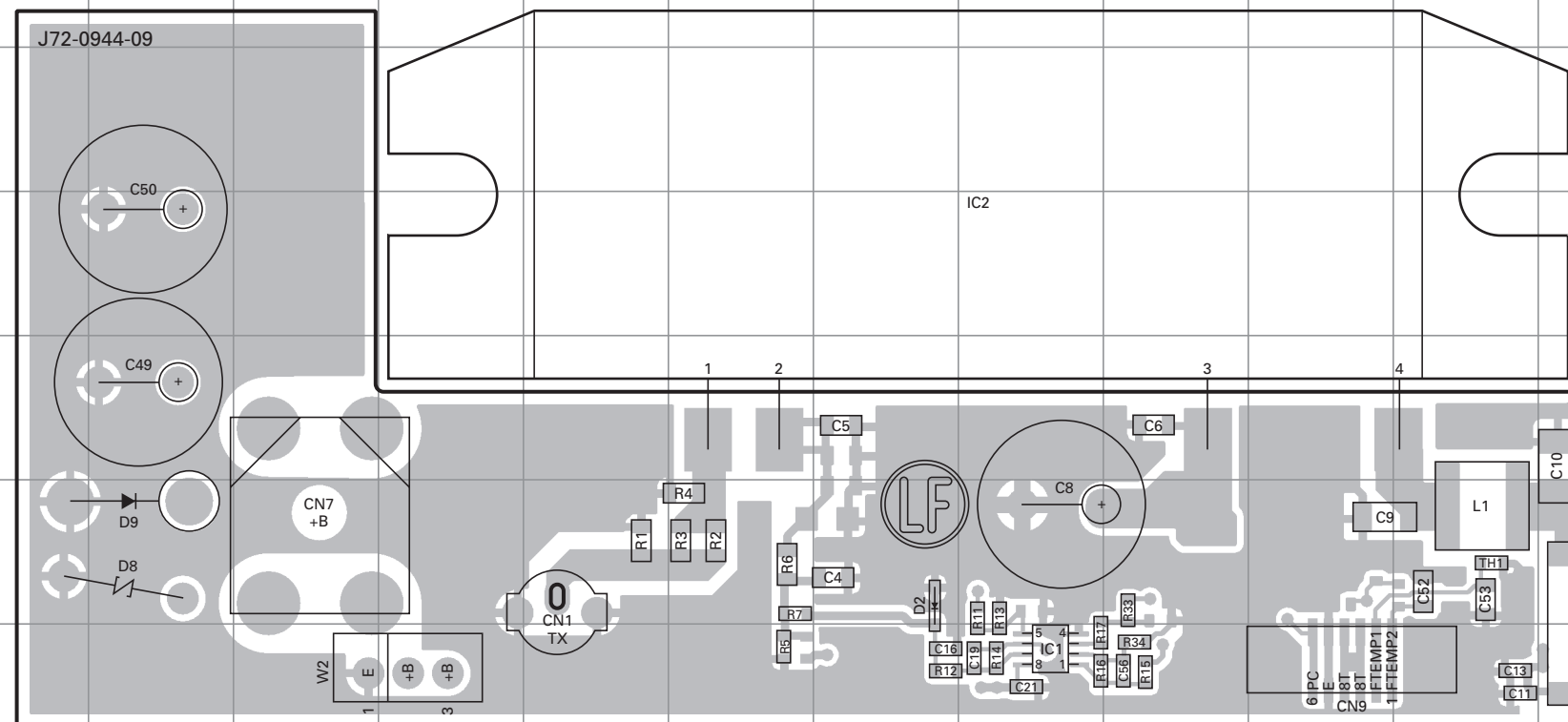
FINAL UNIT (X45-3750-10) : TK-5710(B) Component side view (J72-0944-09)
