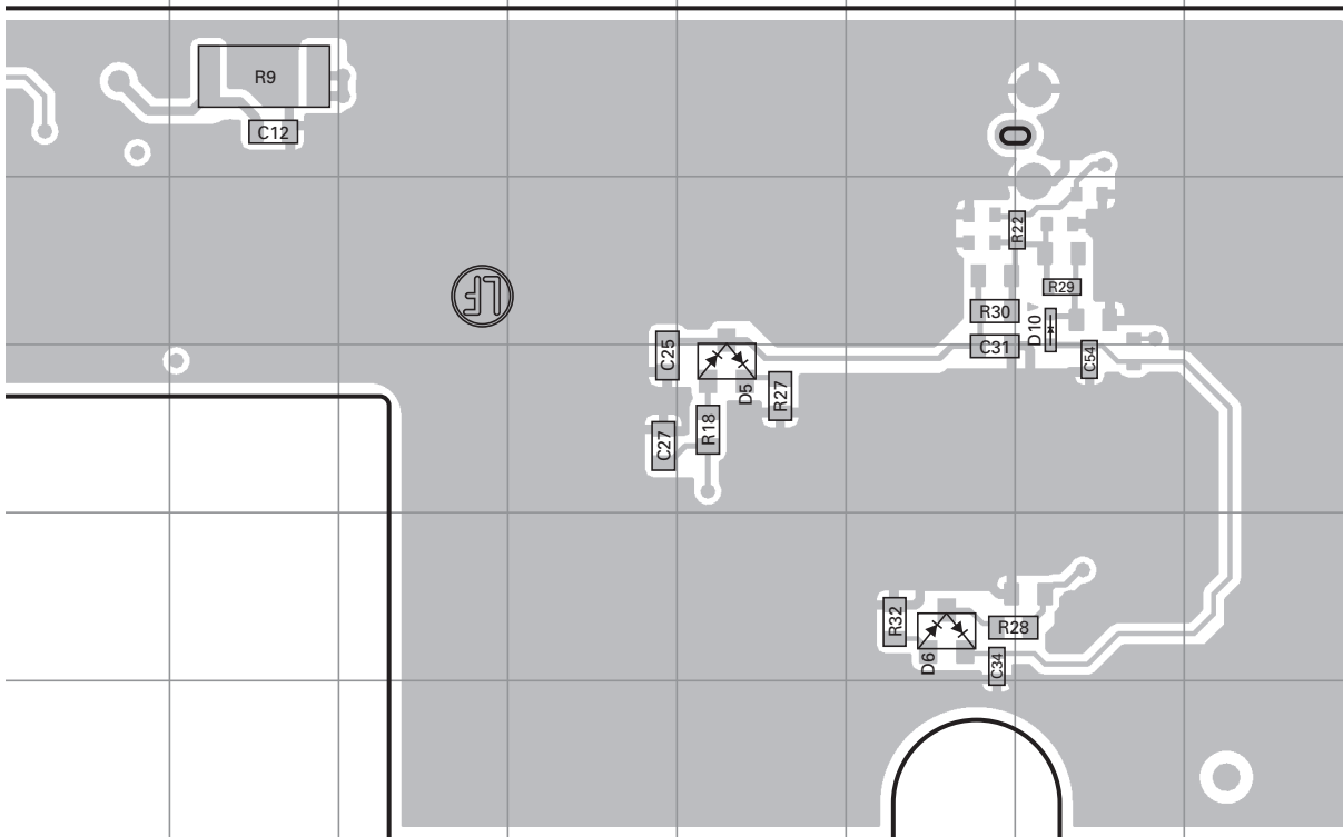
FINAL UNIT (X45-3750-10) : TK-5710(B) Foil side view (J72-0944-09)
