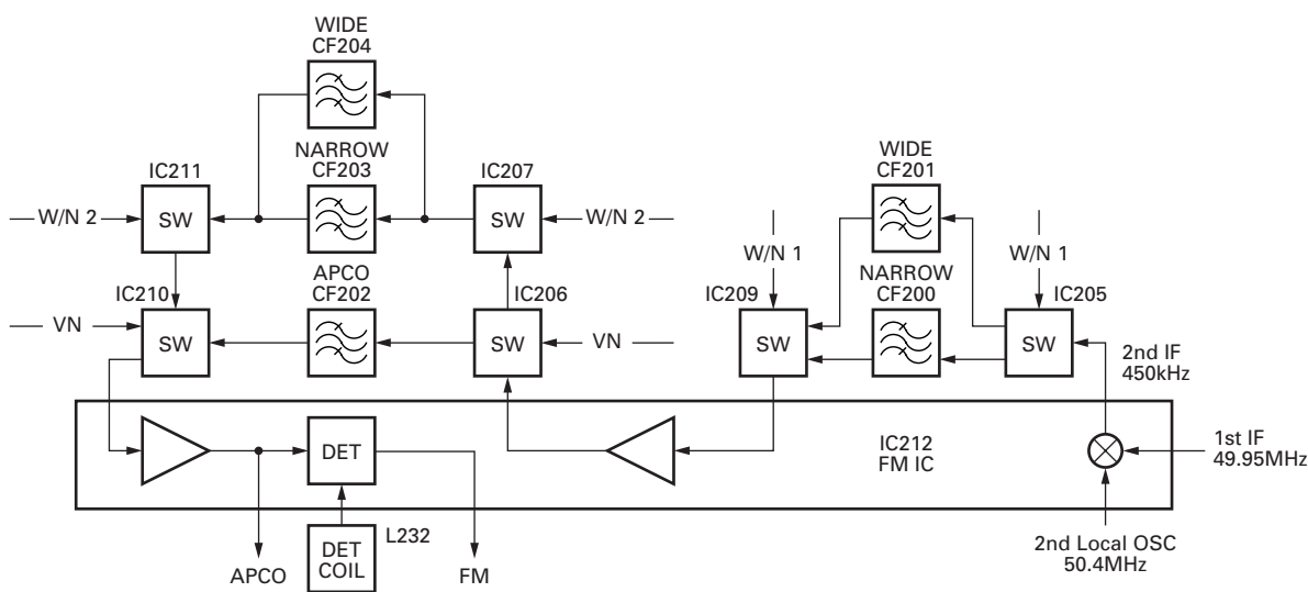
Fig. 4 2nd IF
