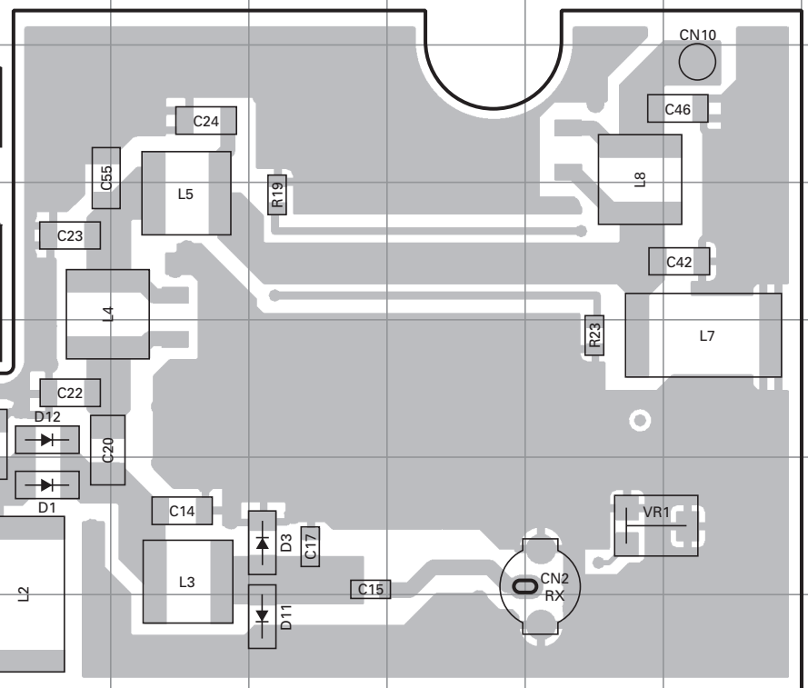
FINAL UNIT (X45-3750-10) : TK-5710(B) Component side view (J72-0944-09)
