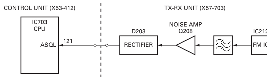
Fig. 6 Squelch circuit
