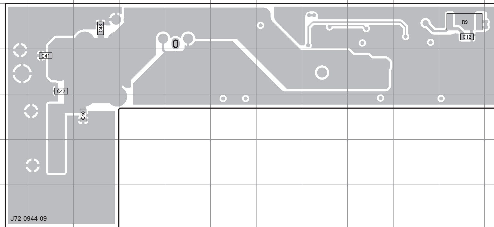
FINAL UNIT (X45-3750-10) : TK-5710(B) Foil side view (J72-0944-09)
