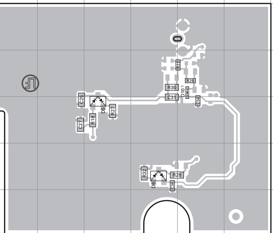
FINAL UNIT (X45-3750-10) : TK-5710(B) Foil side view (J72-0944-09)
